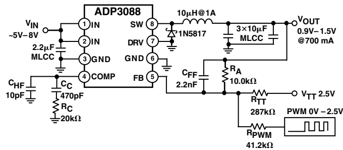
Figure 5. Blackfin DSP Application
